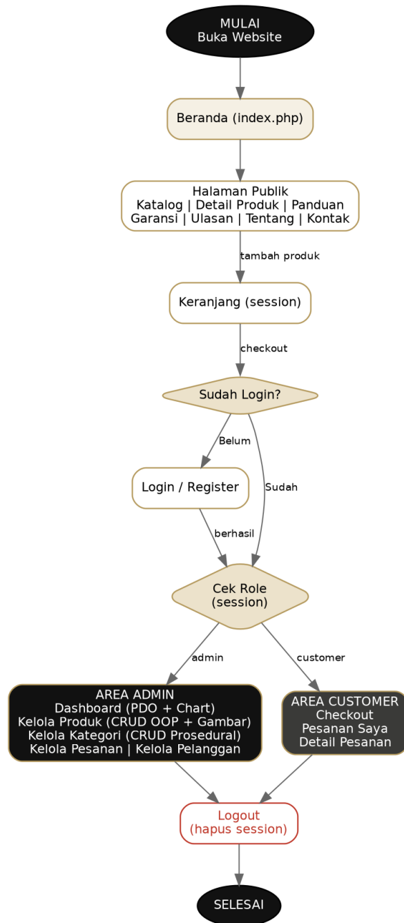
Gambar 1. Flowchart alur navigasi website
