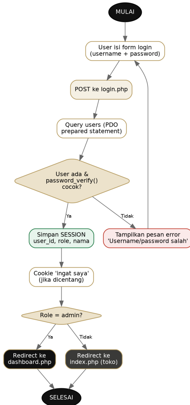
Gambar 2. Flowchart proses login
